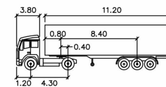
SEMITRAILER 15,5 m
